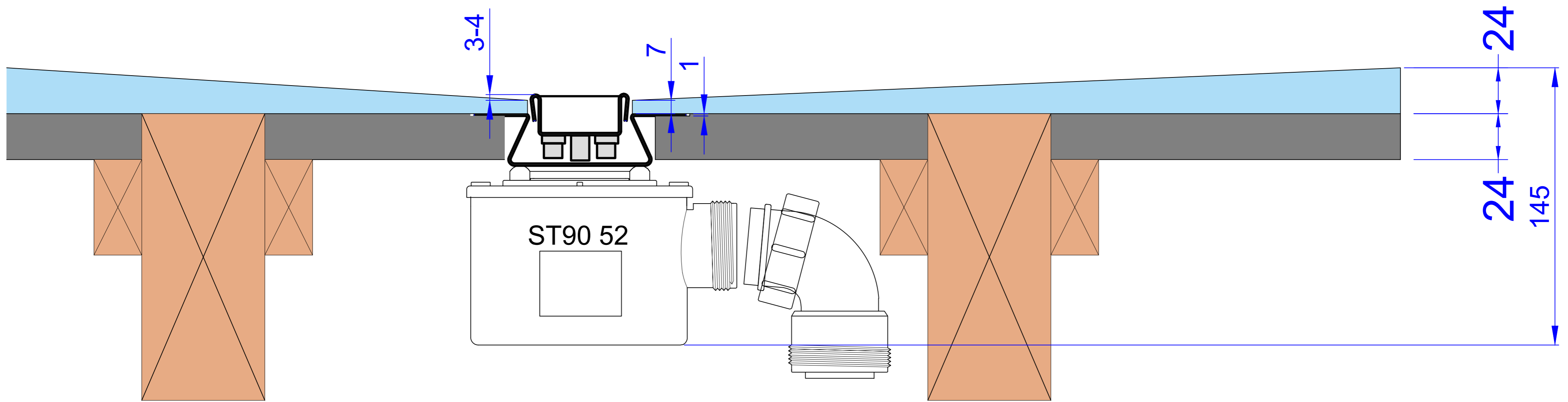
MicroCement floor build up
