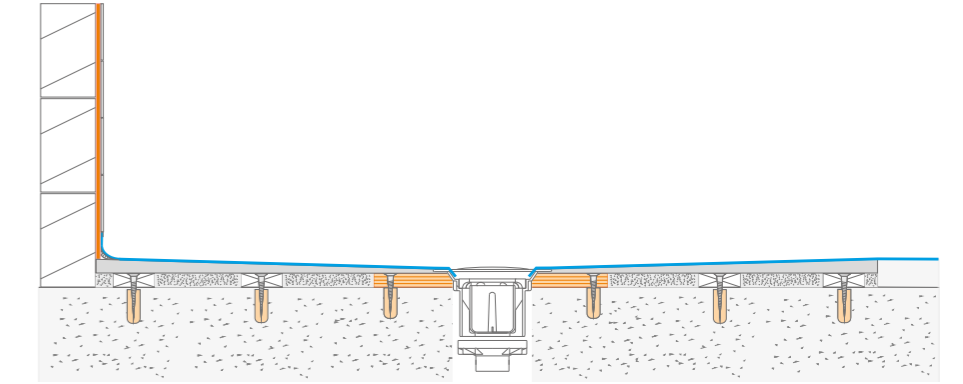
OTL RESIN FORMERS ON A CONCRETE FLOOR
