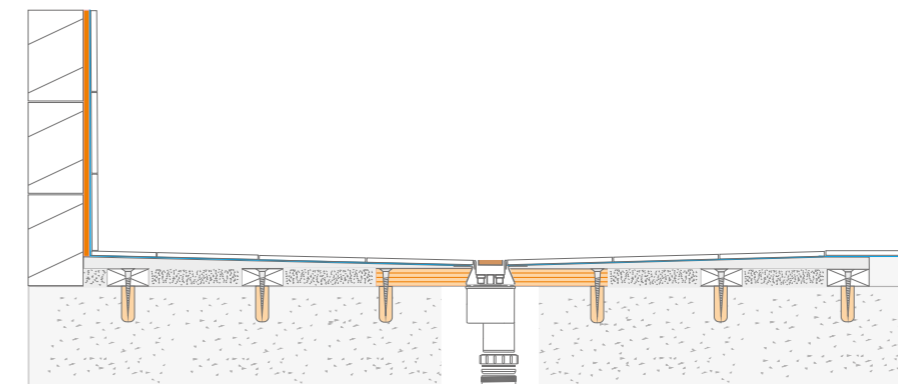
OTL SUPERSLIM CHANNEL ON A CONCRETE FLOOR
